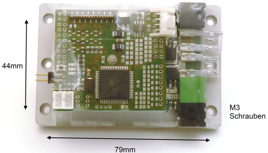
Figure 1: mounting holes
