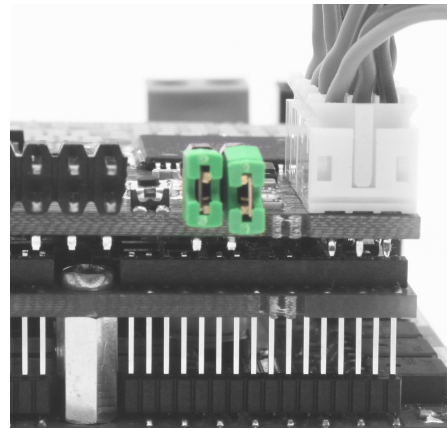
Figure 7: forward BEC voltage to receiver
