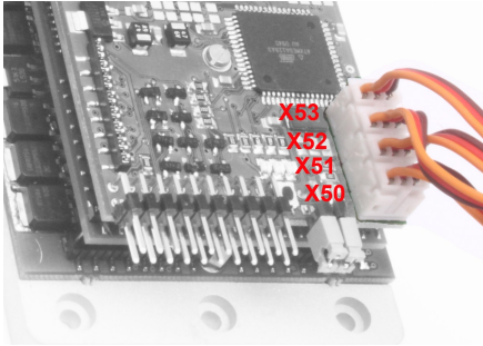
Figure 5: servo cable position
