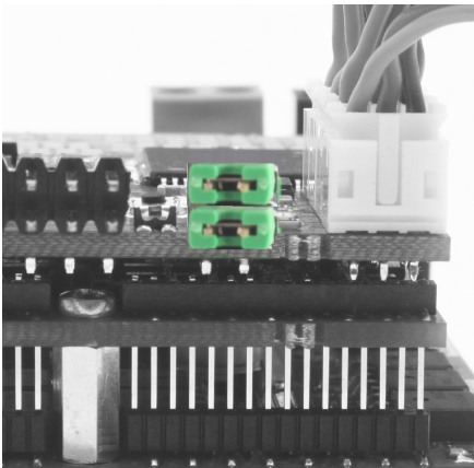
Figure 6: do not forward BEC voltage
